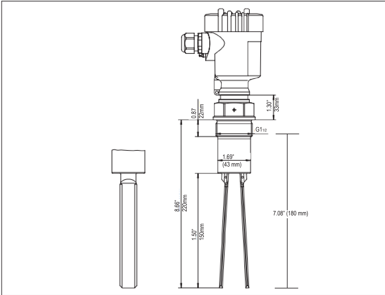
VF-90 Vibrating Fork, 1-1/2" threaded version NPT
